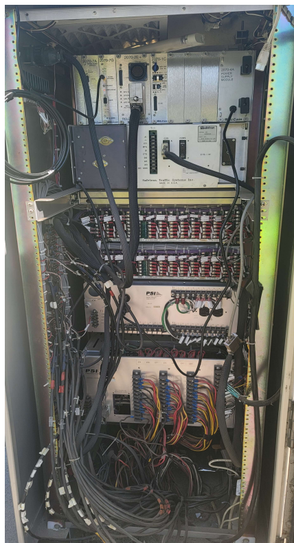
Control cabinet at Geer Rd and Hawkeye Ave with the new controller that was replaced.
